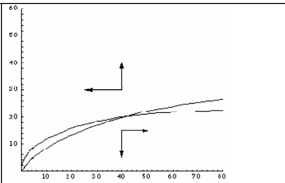
Figure 7B: Phase diagram for the Counterclockwise Treatment
