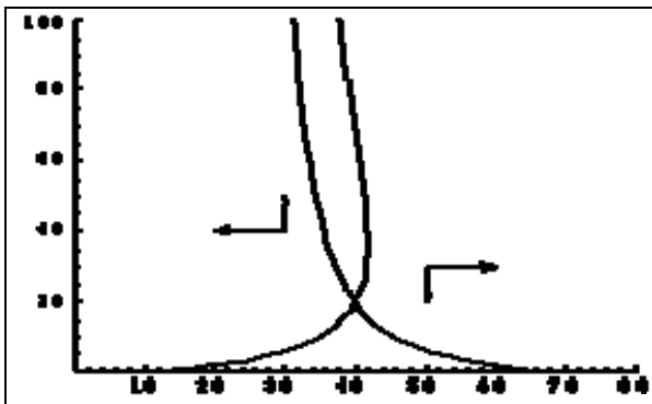
Figure 7A: Phase diagram for the Clockwise Treatment
