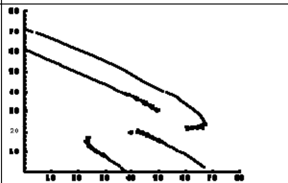
Figure 8B : Simulation of the Counterclockwise treatment with initial prices (24,16), (43,20), (50,30), and (60,22).
