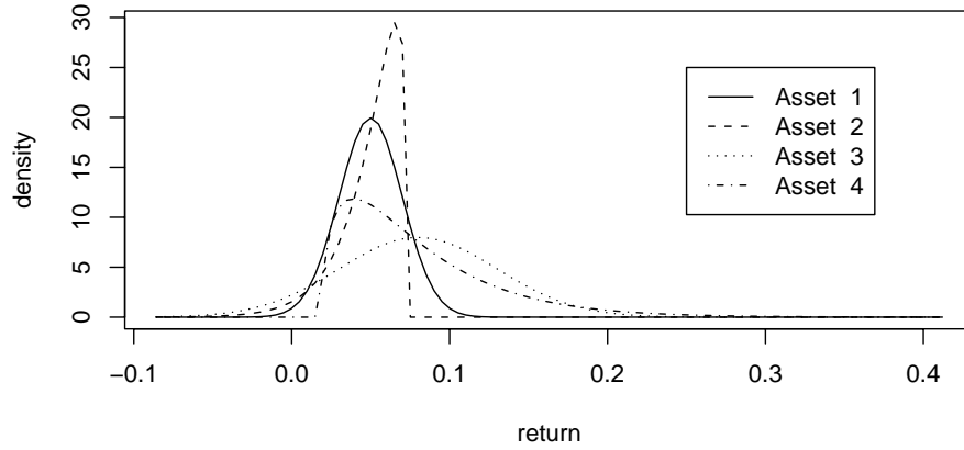
FIGURE 2. Four Asset Densities for Example 1: We will construct portfolios comprised of four independent asset returns with marginal densities illustrated above.
