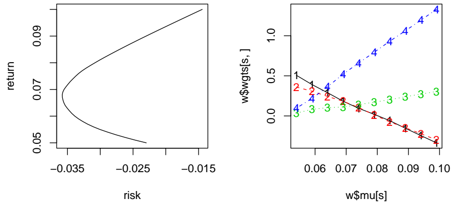
FIGURE 3. The \alpha -risk-return frontier: For the four artificial asset returns series we compute the risk-return frontier according to (3.2) in panel b. The portfolio weights as functions of the required mean return are depicted in Panel c.
