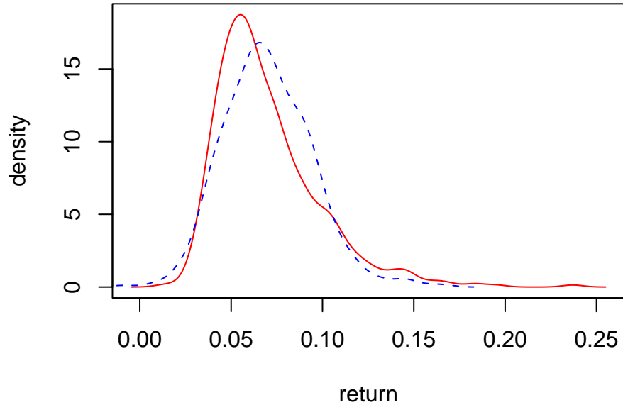
FIGURE 4. Mean-variance vs. \alpha -risk portfolio returns: Based on the data of example 1 we illustrate the estimated density of portfolio returns for the optimal mean-variance portfolio and the optimal \alpha -risk portfolio for required mean return of .07. Note the the solid curve representing the \alpha -risk returns has better performance than the dotted mean-variance density in both tails.
