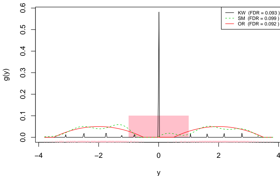
FIGURE 3. One realization of Sun-McLain Model 2. The non-null density is composed of two symmetric, rescaled beta densities supported on \{(-3.5, -0.5) \cup (0.5, 3.5)\} as shown by the solid (red) curve. The rejection region A appears as the shaded rectangle, the Sun and McLain estimate of the non-null density appears as the dashed (green) curve, and the NPMLE estimate of the mixing distribution, including the mass point near zero representing the null distribution, appears as the set of (black) spikes. The sample size for this realization is n = 5000 and \omega = 0.2 .
