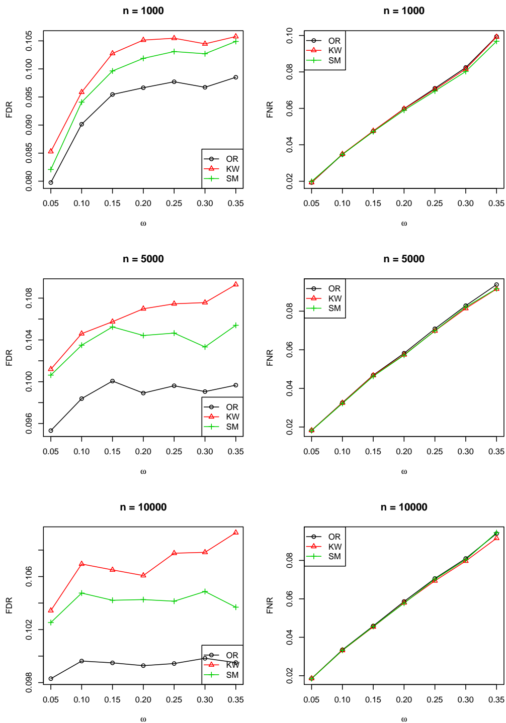
FIGURE 6. FDR and FNR comparison for Sun-McLain Model 3 with symmetric non-null density and heterogeneous scale.
