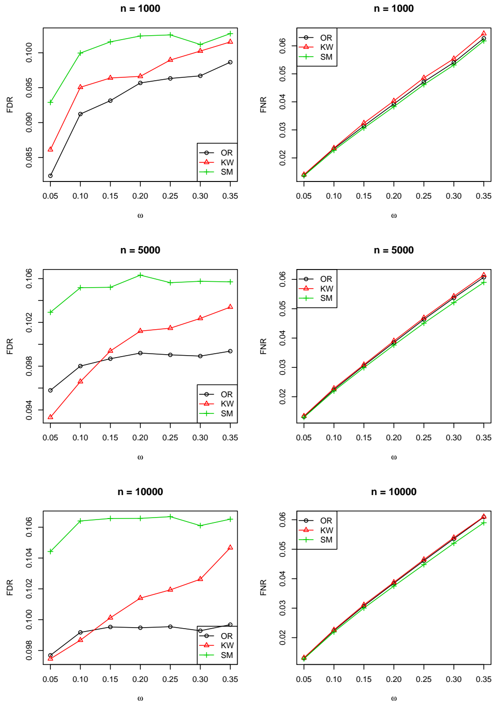
FIGURE 4. FDR and FNR comparison for Sun-McLain Model 2 with symmetric non-null density and homogeneous scale.
