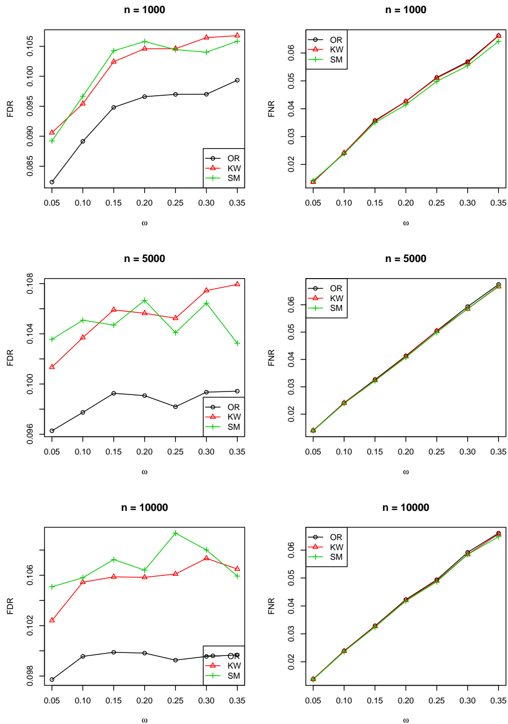
FIGURE 7. FDR and FNR comparison for Sun-McLain Model 3 with asymmetric non-null density and heterogeneous scale.
