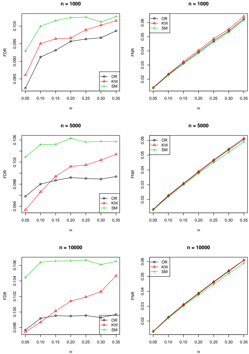
FIGURE 5. FDR and FNR comparison for Sun-McLain Model 2 with asymmetric non-null density and homogeneous scale.
