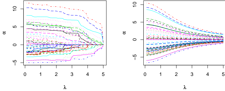
FIGURE 4. Lasso vs Ridge Shrinkage
