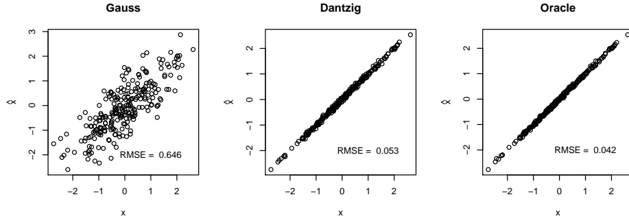
FIGURE 5. The Dantzig Selector Decoding: Estimated values of the signal x plotted versus the true values for three procedures: Gauss ignores the \nu component, Dantzig uses the Dantzig Selector, and Oracle removes \nu as if there were no contamination component.
